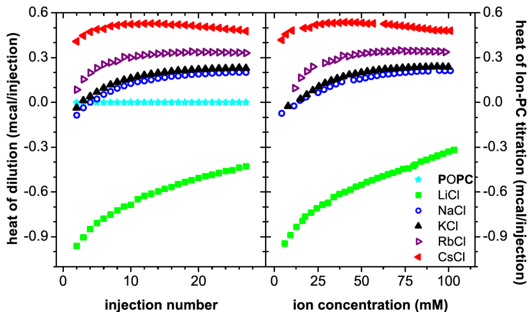
Figure 1: Integrated heats of dilution or reference measurements (left panel) and binding titrations (right panel) corresponding to the heat flow data in Fig. 3 in the main text. Aliquots of 10 \mu l of buffered alkali chlorides (500mM) were injected in HEPES solutions (left) or in 2mM POPC solution (right). The data presented with blue stars are from injecting 10 \mu l aliquots HEPES buffer into 2mM POPC buffered solution.
